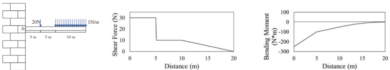
Figure 2: Shear and bending moment diagrams (Johnson-Glauch & Herman, 2017)
