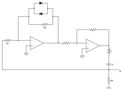
Figure 1. The oscillator
