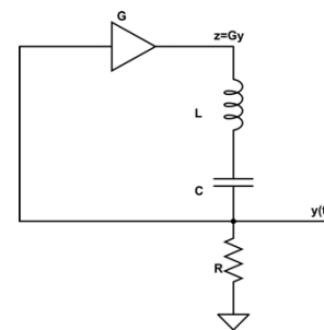
Figure 2. A simple circuit
