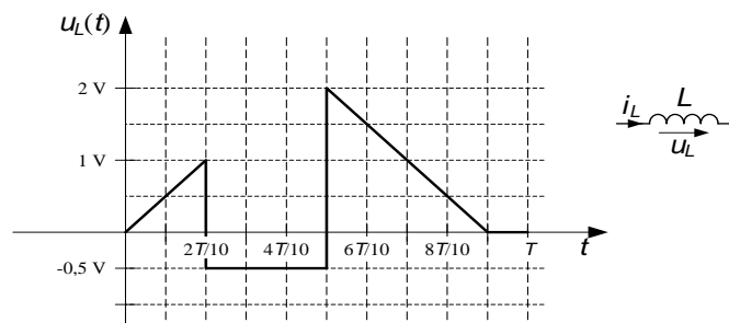
Figure 1: Given sketch of the voltage values
