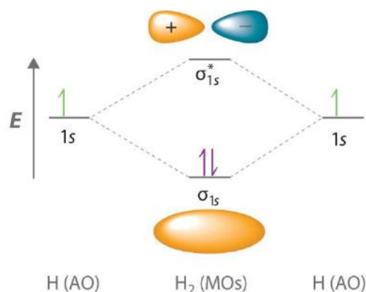
Figure 3: Molecular orbital energy- level diagram for H 2 . The electrons in the 1s orbitals of each hydrogen atom fill the bonding 1s molecular orbital, denoted as \sigma_{1s} (Halpern, n.d.)
