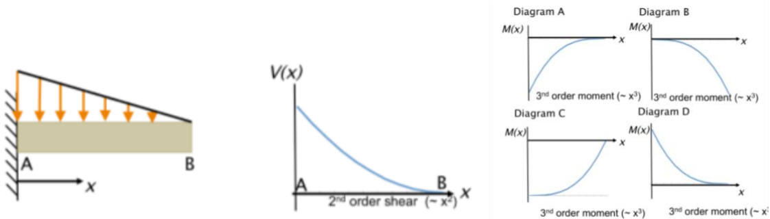
Figure 5: Typical integration task in statics
